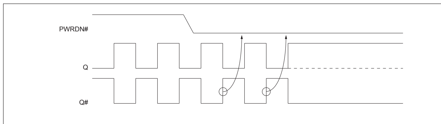
Figure 3. PWRDN# Assertion
