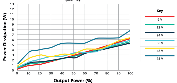
POWER DISSIPATION VS OUTPUT POWER PRQE50W-E12-S28-D (25°C)
