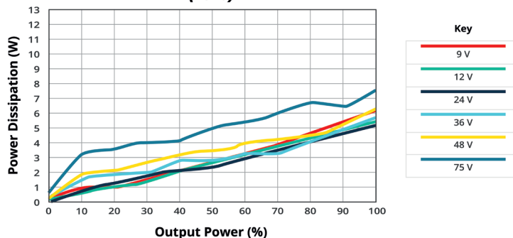
POWER DISSIPATION VS OUTPUT POWER PRQE50W-E12-S24-D (25°C)
