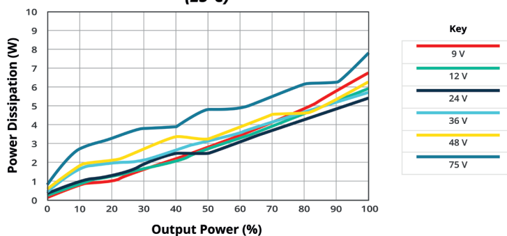
POWER DISSIPATION VS OUTPUT POWER PRQE50W-E12-S15-D (25°C)
