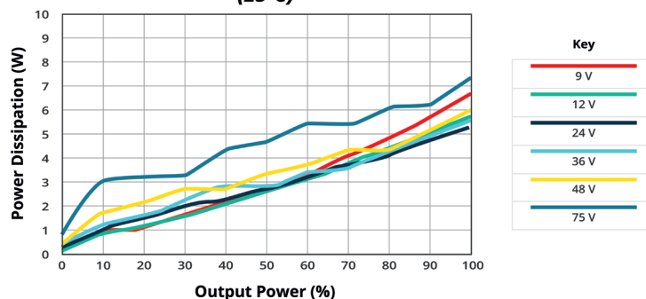
POWER DISSIPATION VS OUTPUT POWER PRQE50W-E12-S12-D (25°C)
