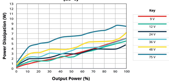
POWER DISSIPATION VS OUTPUT POWER PRQE50W-E12-S48-D (25°C)
