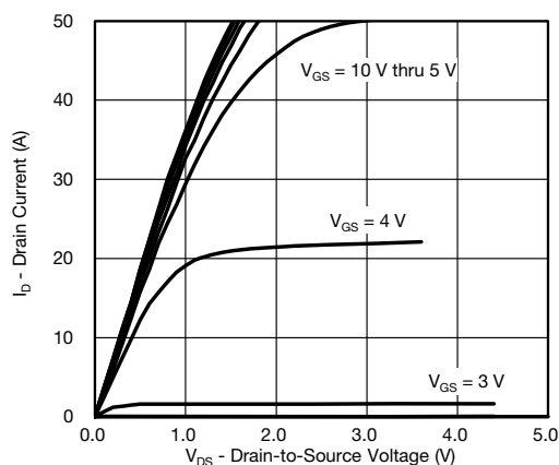
Output Characteristics
