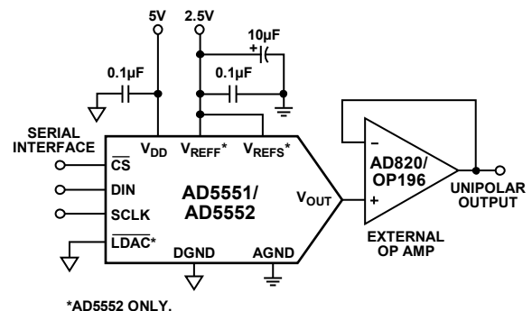
Figure 23. Unipolar Output
