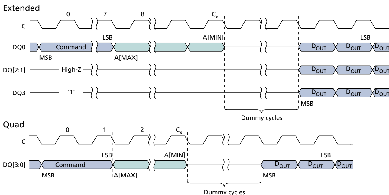
Figure 19: QUAD OUTPUT FAST READ – 6Bh/6Ch 3
