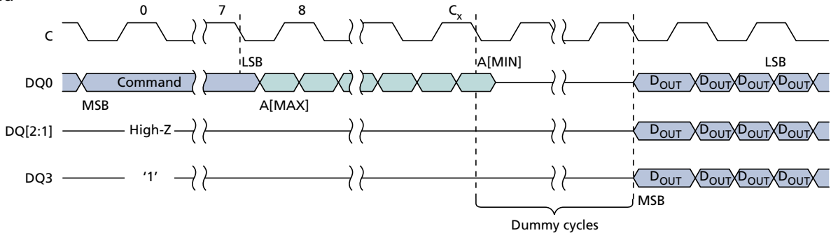
Figure 25: DTR QUAD OUTPUT FAST READ – 6Dh 3
