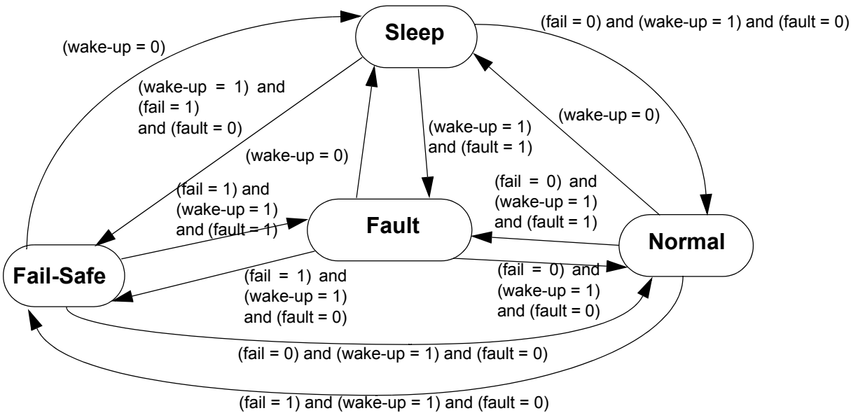
Figure 12. Operating Modes
