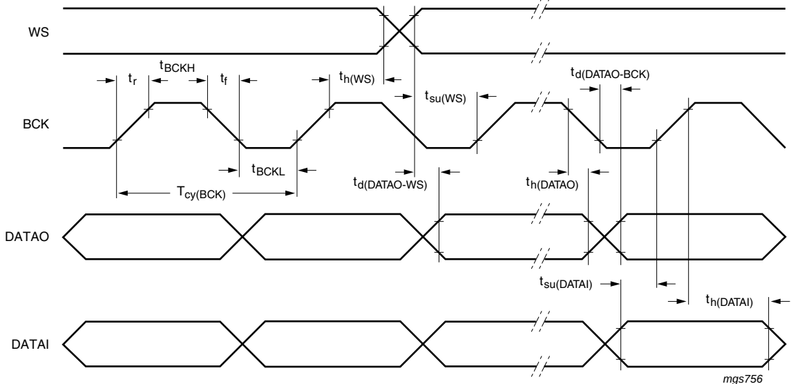
Fig 17. I²S-bus serial interface timing
