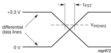
Fig 15. Receiver SE0 width tolerance
