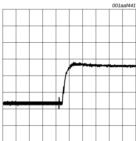
Fig 7. Oscilloscope reading: with resistor and capacitor in the network
