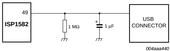
Fig 5. Resistor and electrolytic or tantalum capacitor needed for V_{BUS} sensing
