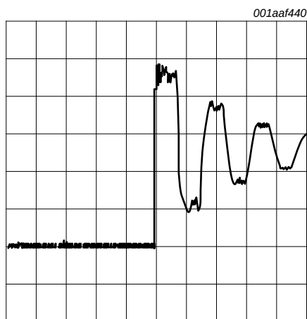
Fig 6. Oscilloscope reading: no resistor and capacitor in the network
