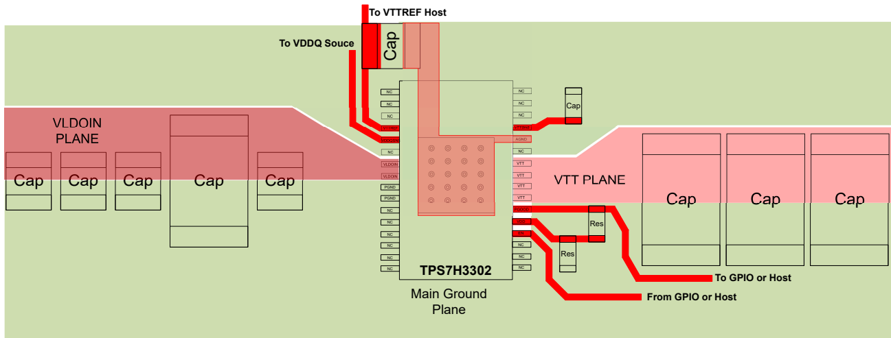
Figure 8-11. Layout Example
