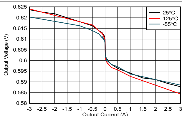
Figure 6-3. Output Voltage vs Output Current
