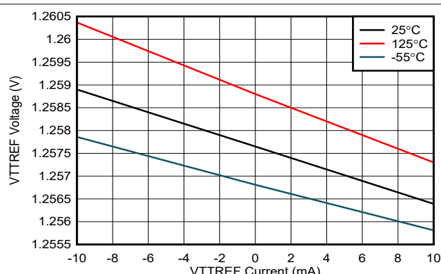
Figure 6-4. Output Voltage vs Output Current
