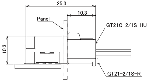
Mating Dimensions Diagram
