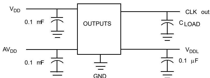
Figure 8. Test Circuit
