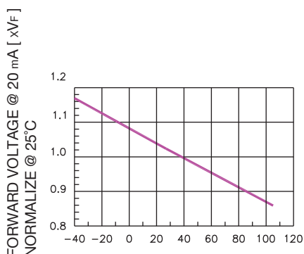
FORWARD VOLTAGE @ 20 mA [ \times 10^4 ] NORMALIZE @ 25°C AMBIENT TEMPERATURE T_a (°C) FORWARD VOLTAGE VS. TEMPERATURE
