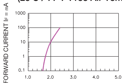
FORWARD CURRENT I_F (mA) FORWARD VOLTAGE V_F (V) FORWARD CURRENT VS. FORWARD VOLTAGE
