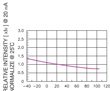
RELATIVE INTENSITY [ \times 10^4 ] @ 20 mA NORMALIZE @ 25°C AMBIENT TEMPERATURE T_a (°C) RELATIVE INTENSITY VS. TEMPERATURE
