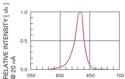
RELATIVE INTENSITY [ \times 10^4 ] @ 20 mA WAVELENGTH (nm) RELATIVE INTENSITY VS. WAVELENGTH
