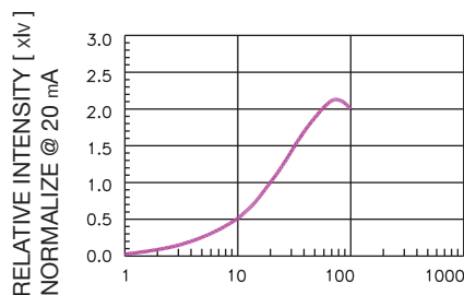
RELATIVE INTENSITY [ \times 10^4 ] NORMALIZE @ 20 mA FORWARD CURRENT I_F (mA) RELATIVE INTENSITY VS. FORWARD CURRENT
