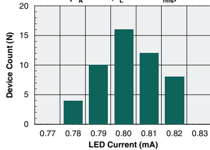
Typical I_F for Switch Operation ( T_A=25^\circ\text{C} , I_L=500\text{mA}_{\text{rms}} )
