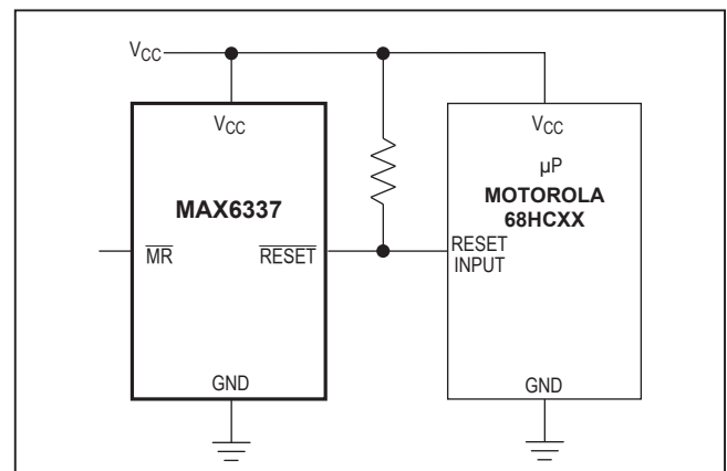
Figure 1. Interfacing to μPs with Bidirectional Reset Pins
