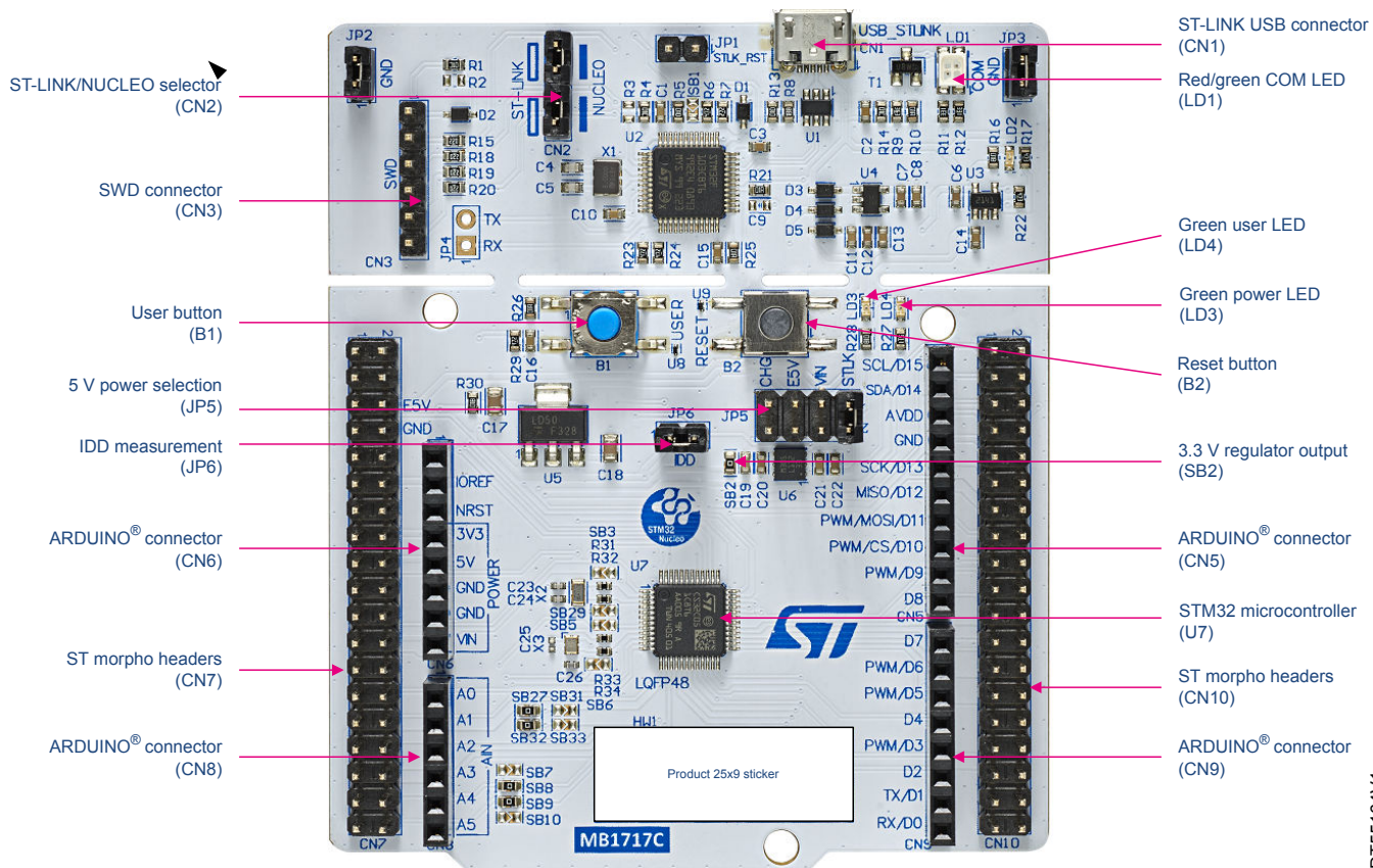
Figure 3. Nucleo-64 PCB top side
