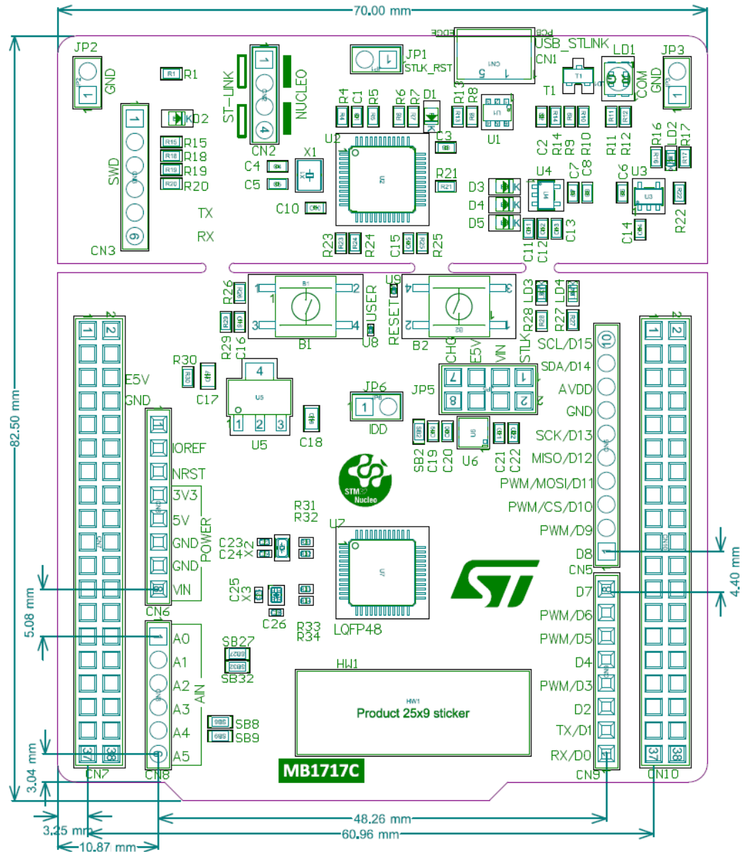
Figure 5. STM32 Nucleo-64 board mechanical dimensions (in millimeters)
