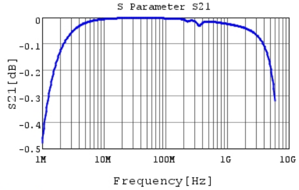
GCM1885C1H472JA16 S21 DCOV, 25degC
