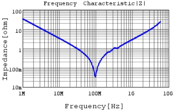
GCM1885C1H472JA16 |Z| DCOV, 25degC
