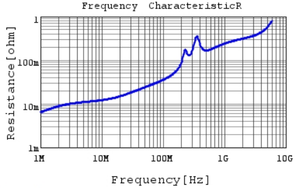
GCM1885C1H472JA16 R DCOV, 25degC
