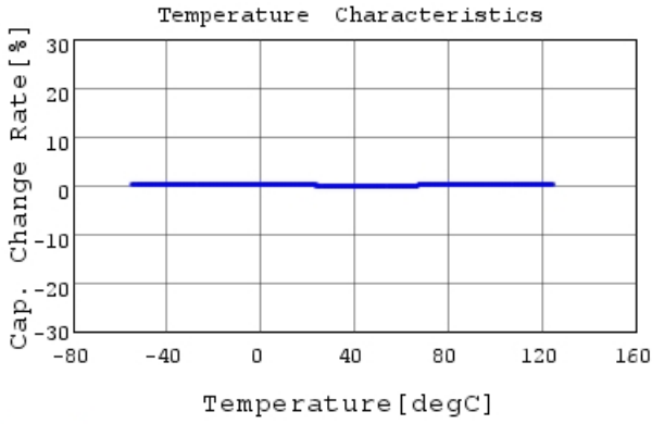
GCM1885C1H472JA16 C-Temp. capchange, DCOV, 1
