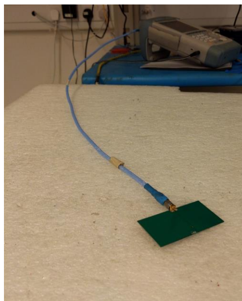
VNA Set-up
