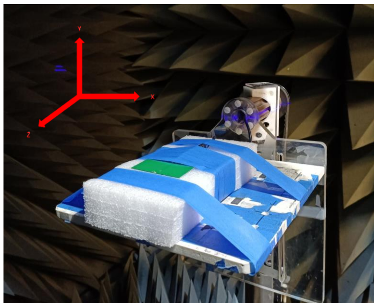
Chamber Set-up
