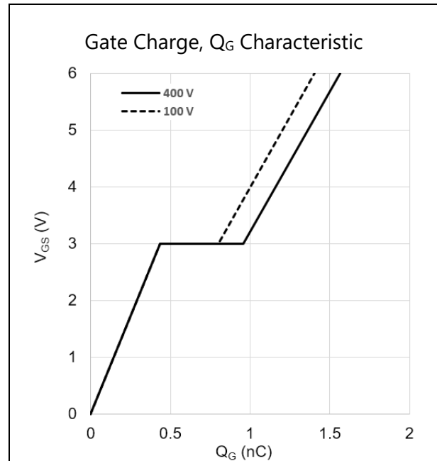
Figure 6: Typical V_{GS} vs. Q_G @ V_{DS} = 100, 400 V
