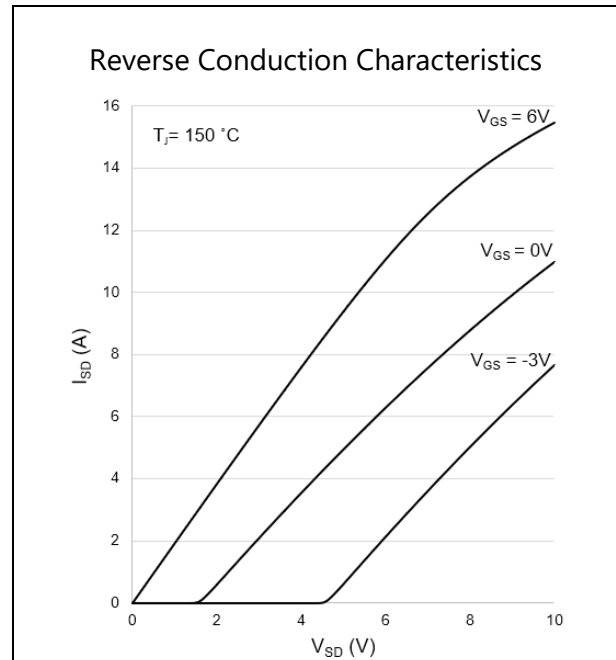
Figure 10: Typical I_{SD} vs. V_{SD} @ T_J = 150\text{ }^{\circ}\text{C}
