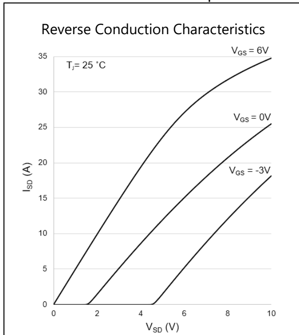
Figure 9: Typical I_{SD} vs. V_{SD} @ T_J = 25\text{ }^{\circ}\text{C}
