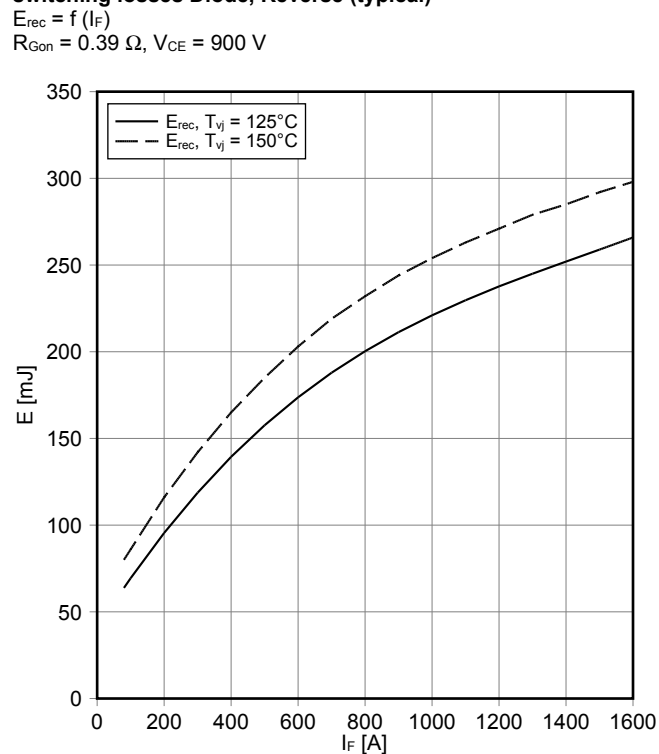
Schaltverluste Diode, Revers (typisch) switching losses Diode, Reverse (typical) E_{rec} = f(I_F) R_{Gon} = 0.39 \Omega , V_{CE} = 900 V
