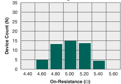
Typical On-Resistance Distribution (N=50, I_L=150\text{mA} )
