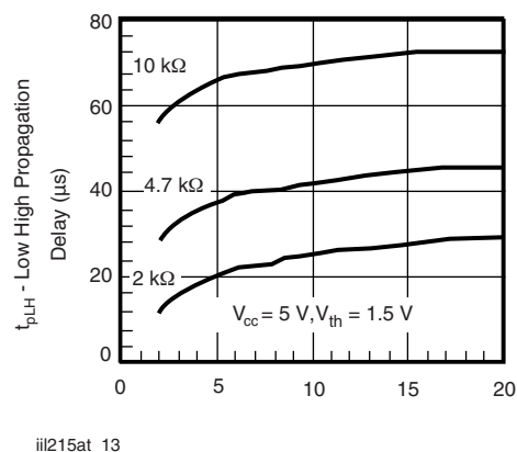
Fig. 13 - Low to High Propagation Delay vs. LED Current and Load Resistor
