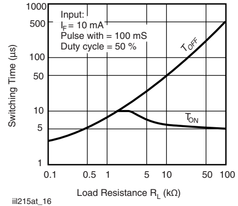
Fig. 16 - Typical Switching Times vs. Load Resistance
