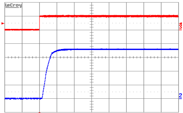
Figure 7. Turn-on transient at full rated load current (resistive) plus 30,000 \mu\text{F} at V_{in} = 48 \text{ V} , triggered via ON/OFF pin. Top trace: ON/OFF signal (5 V/div.). Bottom trace: Output voltage (0.5 V/div.). Time scale: 5 ms/div.
