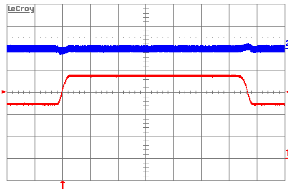
Figure 8. Output voltage response to load current step-change (12.5 A–18.75 A–12.5 A) at V_{in} = 48 \text{ V} . Top trace: output voltage (200 mV/div.). Bottom trace: load current (5 A/div.). Current slew rate: 0.1 A/µs. C_o = 1 \mu\text{F cer} + 10 \mu\text{F tant} . Time scale: 0.2 ms/div.
