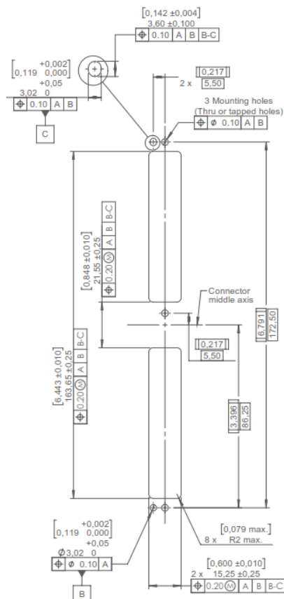
Plug - Shown from the Front Side
