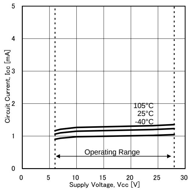
Figure 1. Circuit Current
