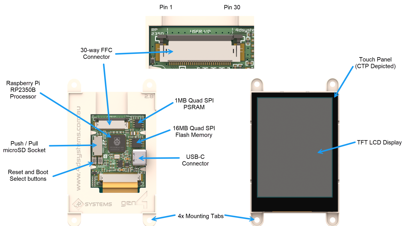
Hardware Layout (2.8" CTP Module depicted)
