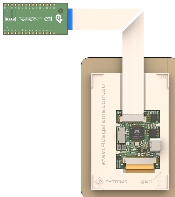
gen4-RP2350 Breakout Back
