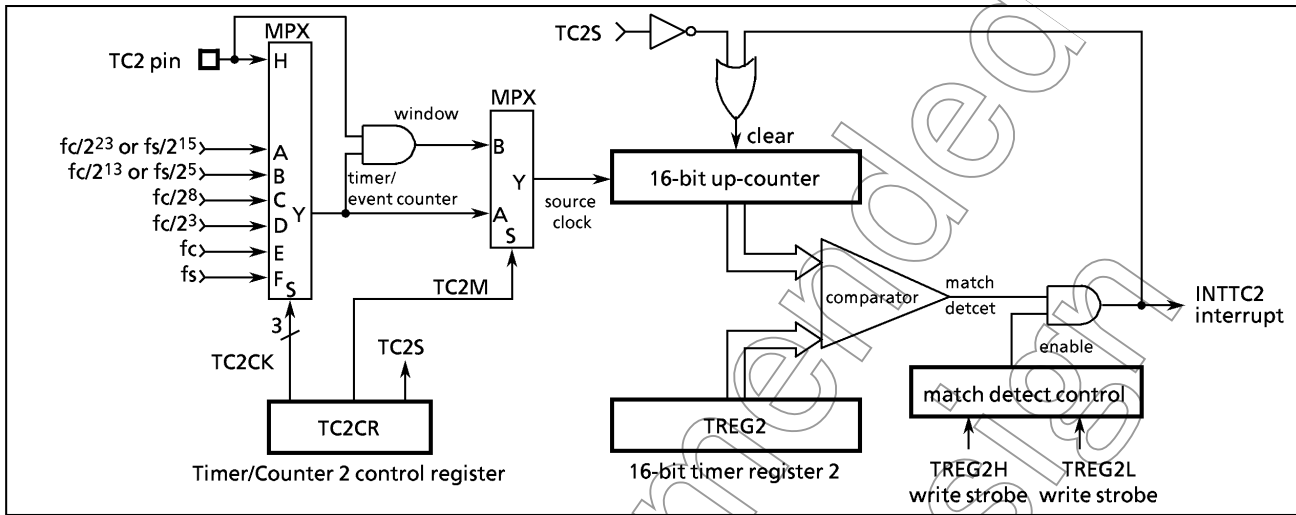
Figure 2-23. Timer/Counter 2 (TC2)
