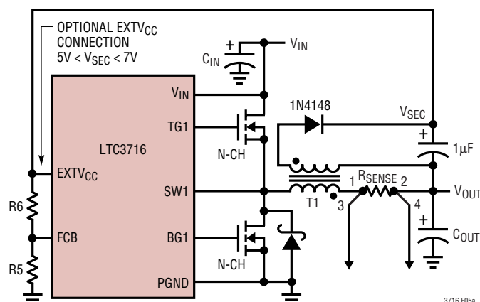
Figure 5a. Secondary Output Loop with EXTVCC Connection
