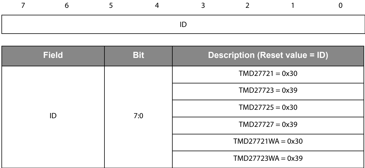
Figure 44: ID Register
