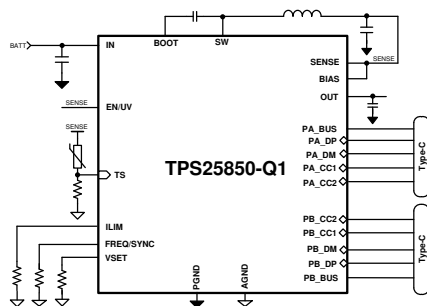
Simplified Schematic TPS25850-Q1
