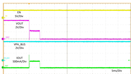
Figure 11-28. OUT short to 5.1- \Omega Load
