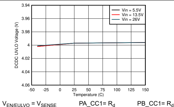
Figure 8-7. DCDC UVLO Threshold
