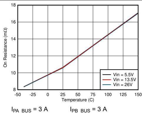
Figure 8-11. Low-side MOSFET on Resistance vs Junction Temperature
