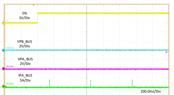
Figure 11-20. Rd Assert
