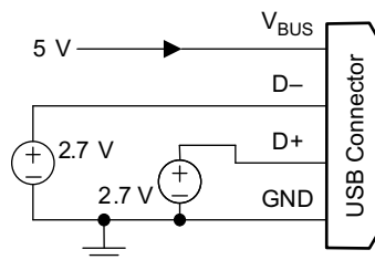
Figure 10-22. Divider 3 Mode
