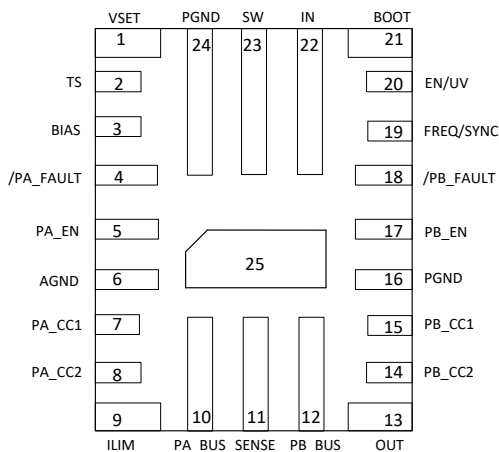
Figure 7-3. TPS25852-Q1 RPQ Package 25-Pin (QFN) Top View
