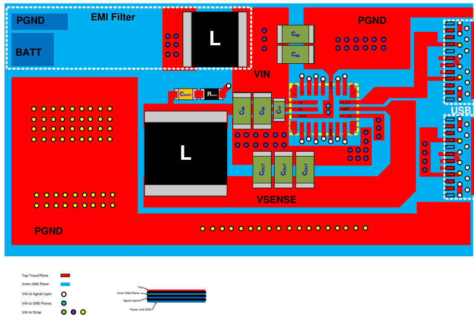
Figure 13-1. Layout Example
