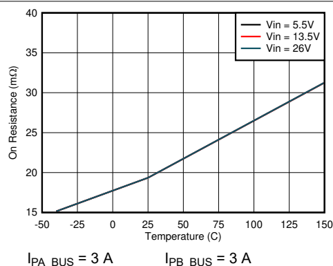
Figure 8-10. High-side MOSFET on Resistance vs Junction Temperature
