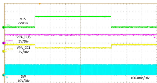
Figure 11-30. Thermal Sensing - NTC Temperature WARM Behavior
