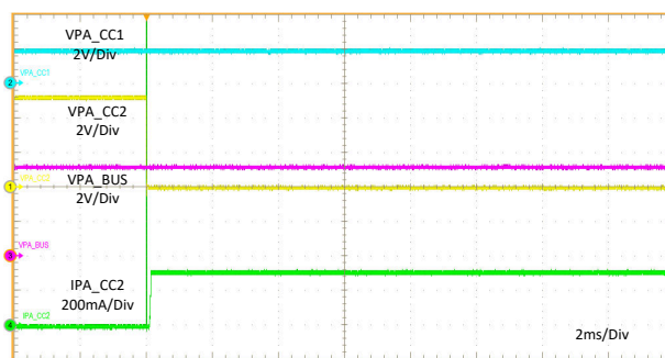
Figure 11-27. PA_CC2 Hot Short to GND
