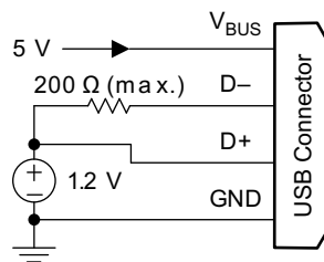
Figure 10-23. 1.2-V Mode
