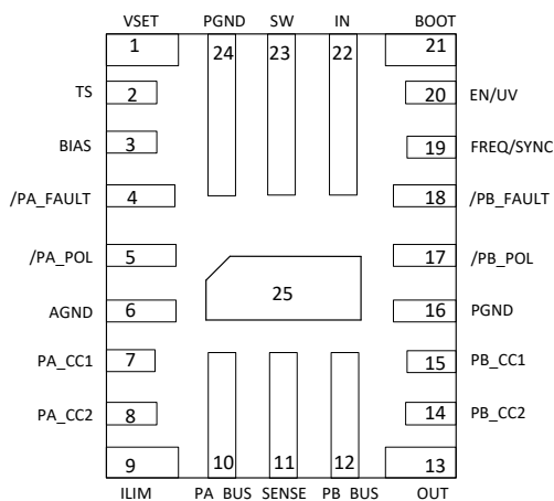
Figure 7-2. TPS25851-Q1 RPQ Package 25-Pin (QFN) Top View
