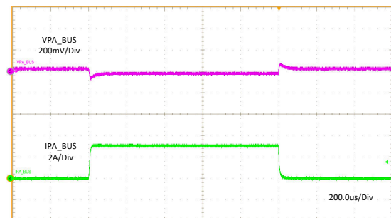
Figure 11-5. Load Regulation
