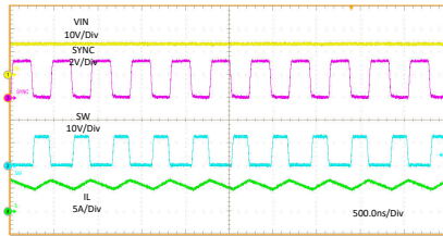
Figure 10-9. Synchronizing to External 2.2-MHz Clock
