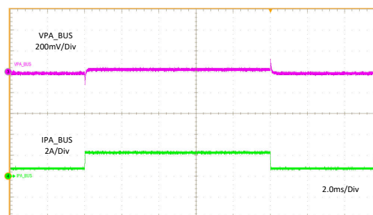
Figure 11-9. Load Transient Without Cable Compensation
