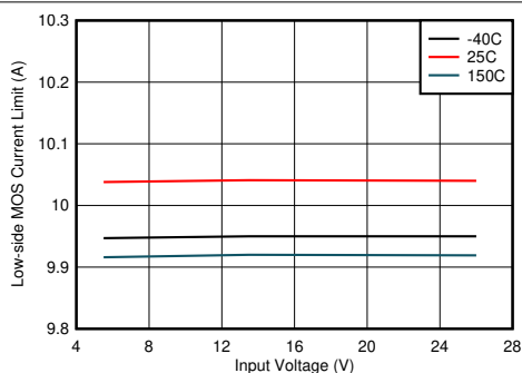
Figure 8-9. Low-side Current Limit vs Input Voltage
