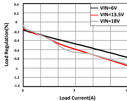
Figure 11-5. Load Regulation
