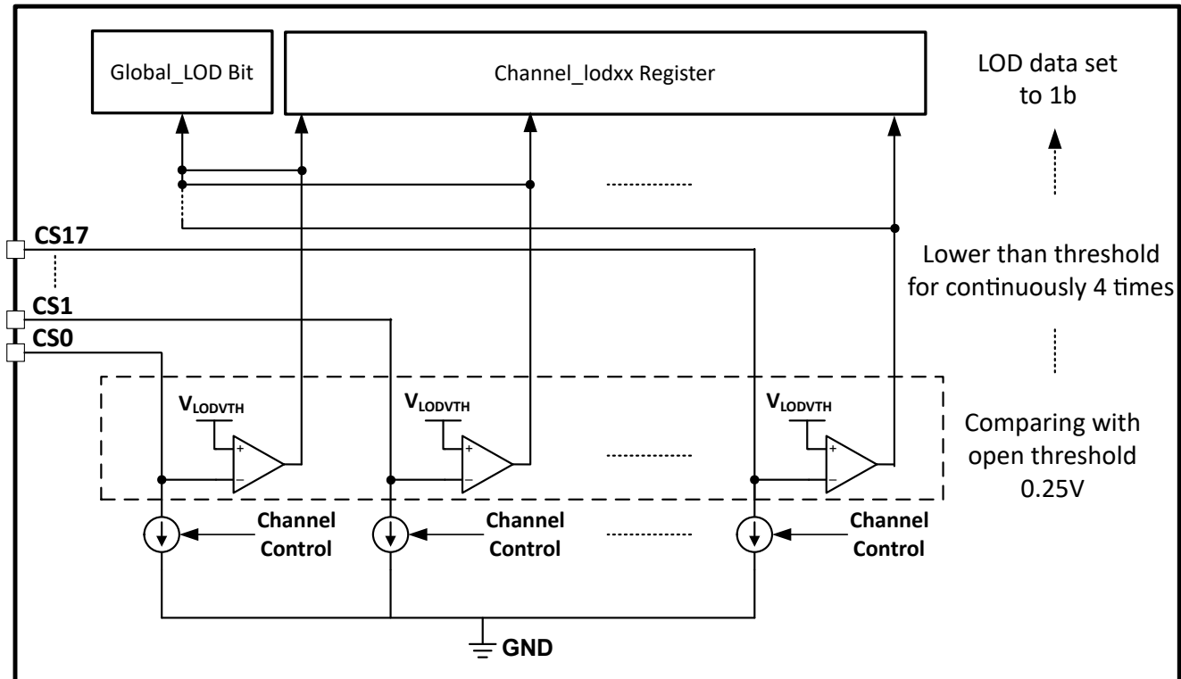
Figure 8-11. LOD Circuits
