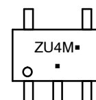
SC-88A CASE 419A-02
