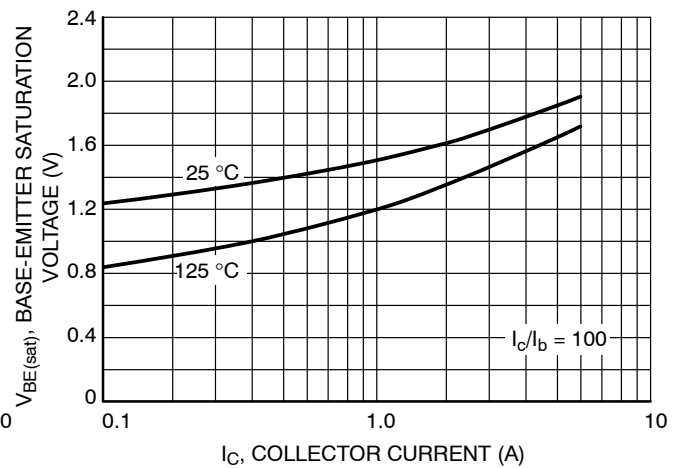
Figure 5. Base-Emitter Saturation Voltage
