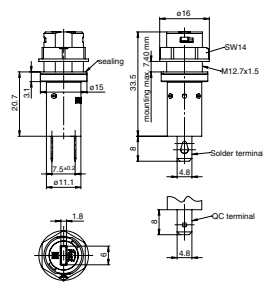
IP67 / Variants 3101.0120 and 3101.0320
