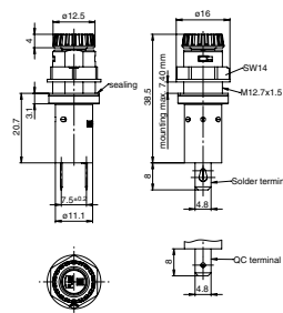
IP67 / Variants Fingergrasp 3101.0125 and 3101.0325
