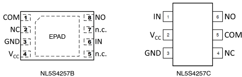
Figure 1. Pin Assignments (Top View)
