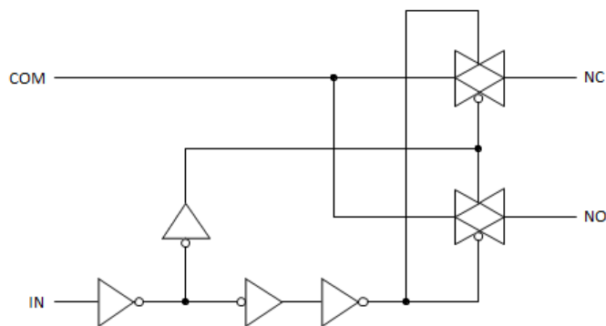
Figure 2. Analog Symbol
