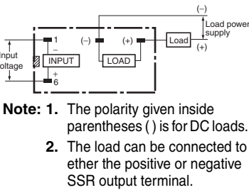
Terminal Arrangement/Connections (Bottom View)
