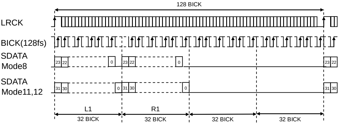
Figure 32. Mode 8/11/12 Timing
