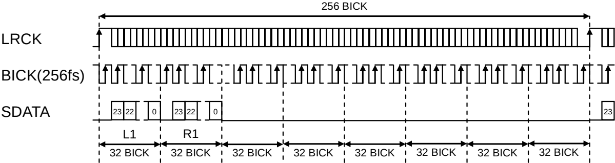
Figure 37. Mode 16 Timing
