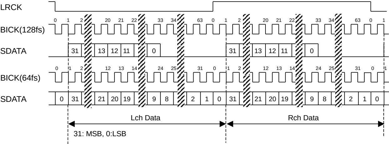
Figure 31. Mode 7 Timing
