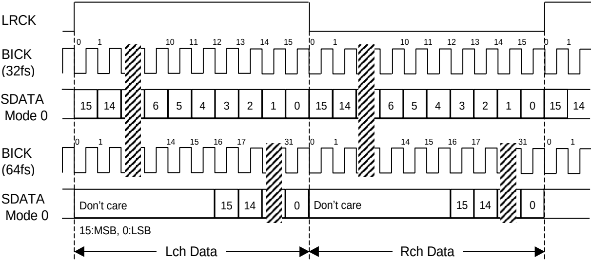
Figure 25. Mode 0 Timing
