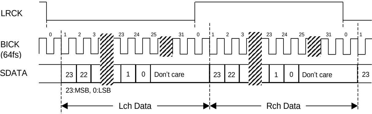
Figure 28. Mode 3 Timing
