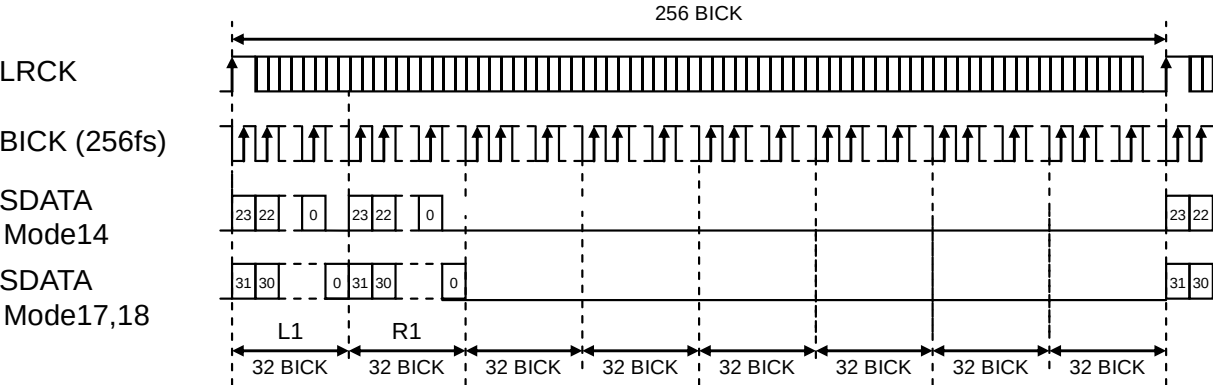
Figure 35. Mode 14/17/18 Timing
