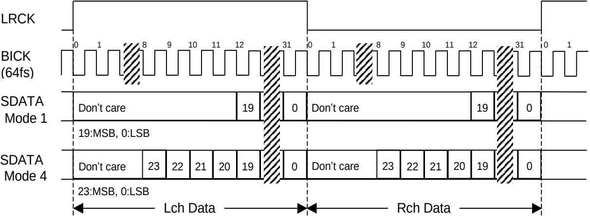
Figure 26. Mode 1, 4 Timing
