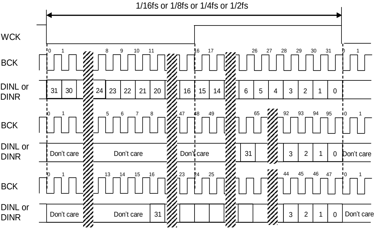
Figure 49. EXDF Mode Timing
