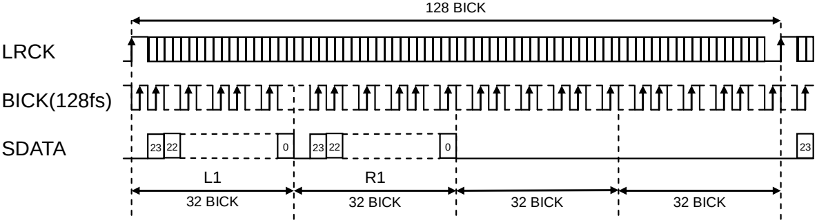
Figure 34. Mode 10 Timing
