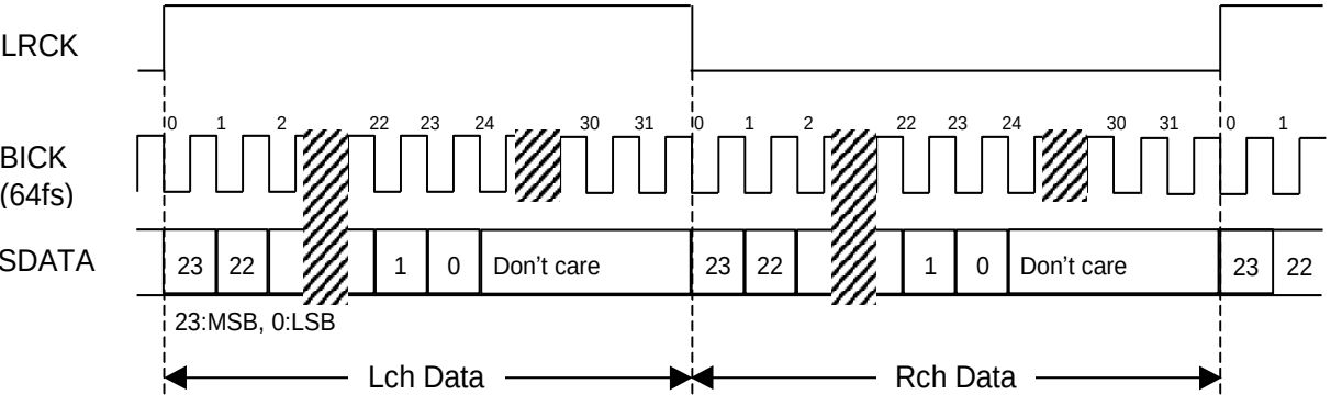
Figure 27. Mode 2 Timing
