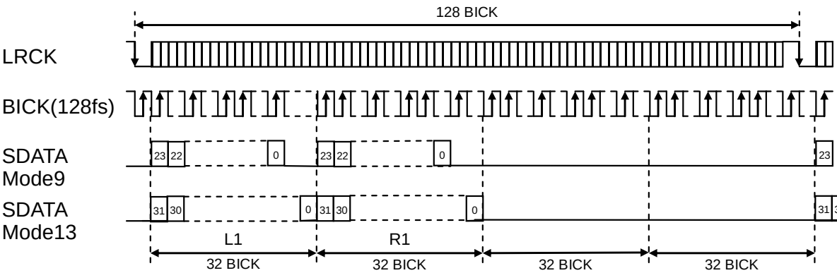
Figure 33. Mode 9/13 Timing
