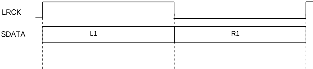
Figure 41. Data Slot in Normal Mode
