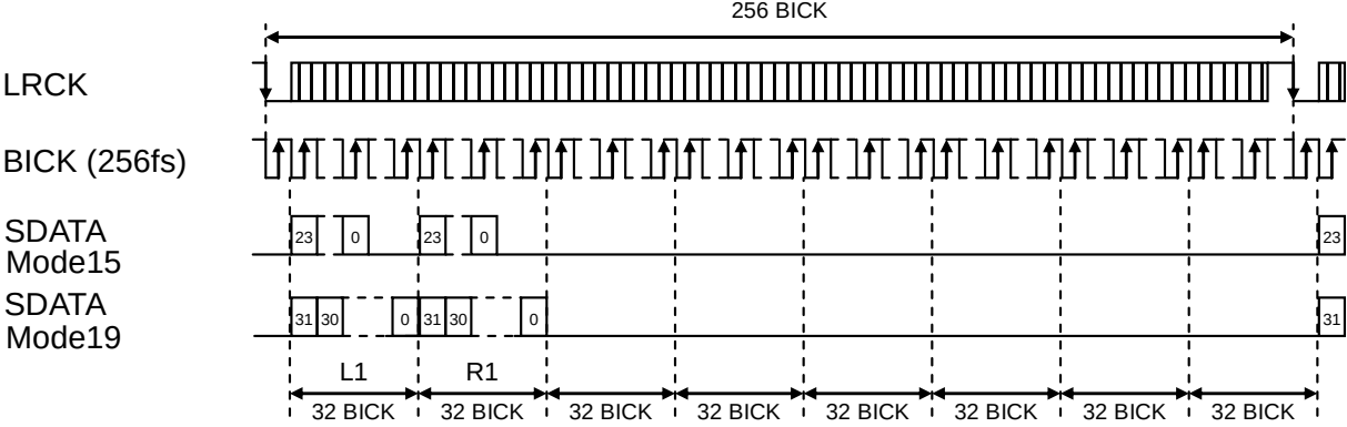
Figure 36. Mode 15/19 Timing
