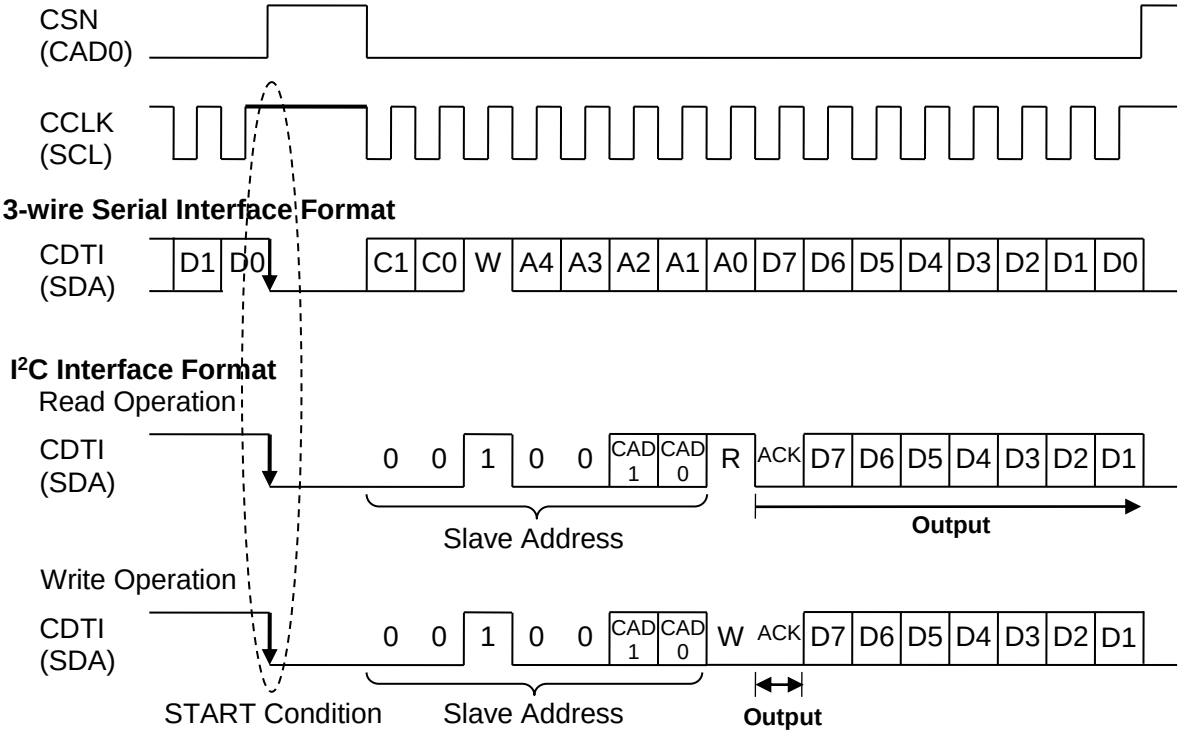
Figure 63. Comparison of 3-wire Serial and I 2 C Interface Timing
