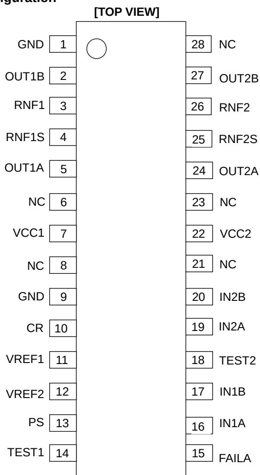
Figure 3. Pin Configuration
