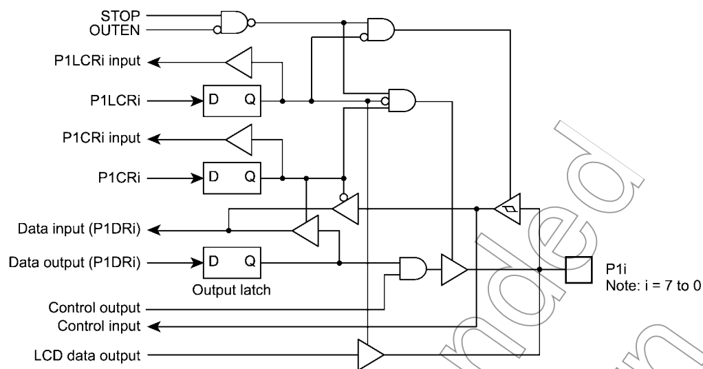
Figure 5-2 Port P1
