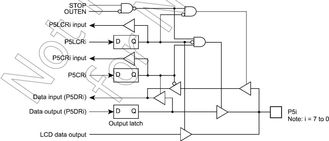
Figure 5-5 Port P5
