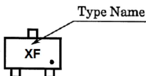
Fig. 10.6 Marking RN1106MFV
