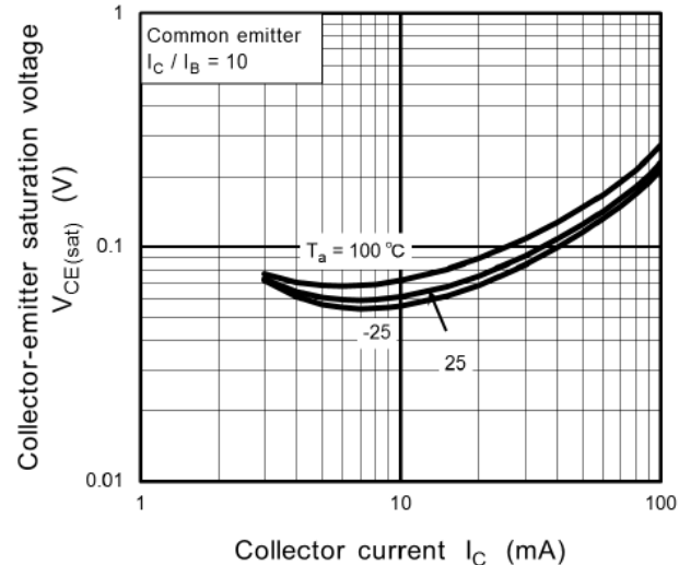
Fig. 11.19 RN1101MFV V_{CE(sat)} - I_C
