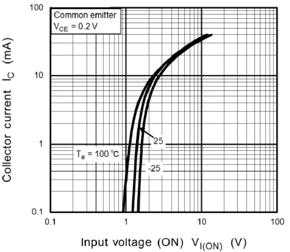
Fig. 11.2 RN1102MFV I_C - V_{I(ON)}
