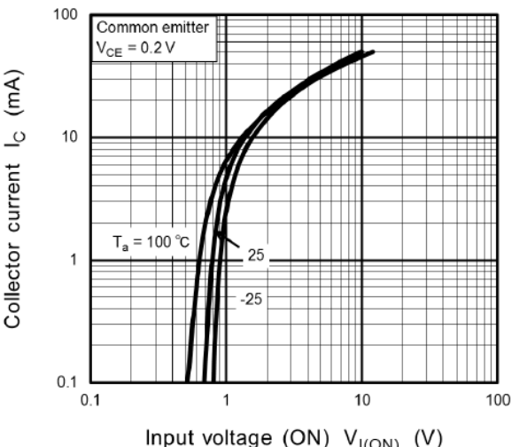
Fig. 11.6 RN1106MFV I_C - V_{I(ON)}
