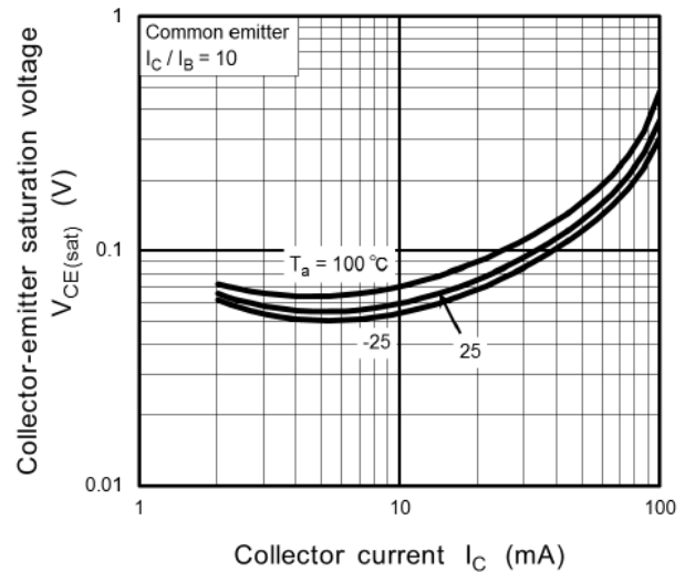
Fig. 11.20 RN1102MFV V_{CE(sat)} - I_C
