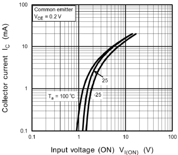
Fig. 11.4 RN1104MFV I_C - V_{I(ON)}
