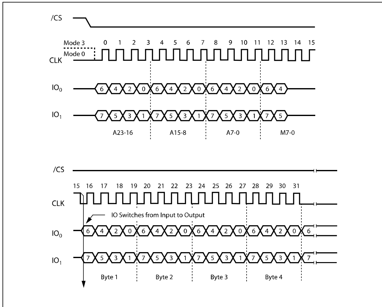
Figure 12b. Fast Read Dual Input/Output Instruction Sequence Diagram (M7-0 = Axxh)
