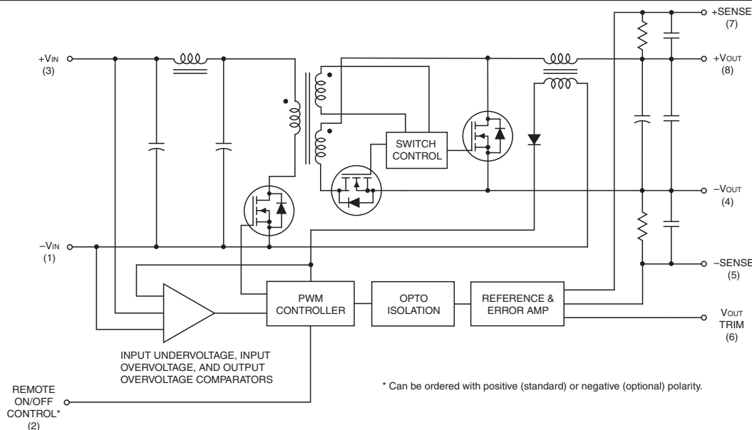
Figure 1. Simplified Schematic
