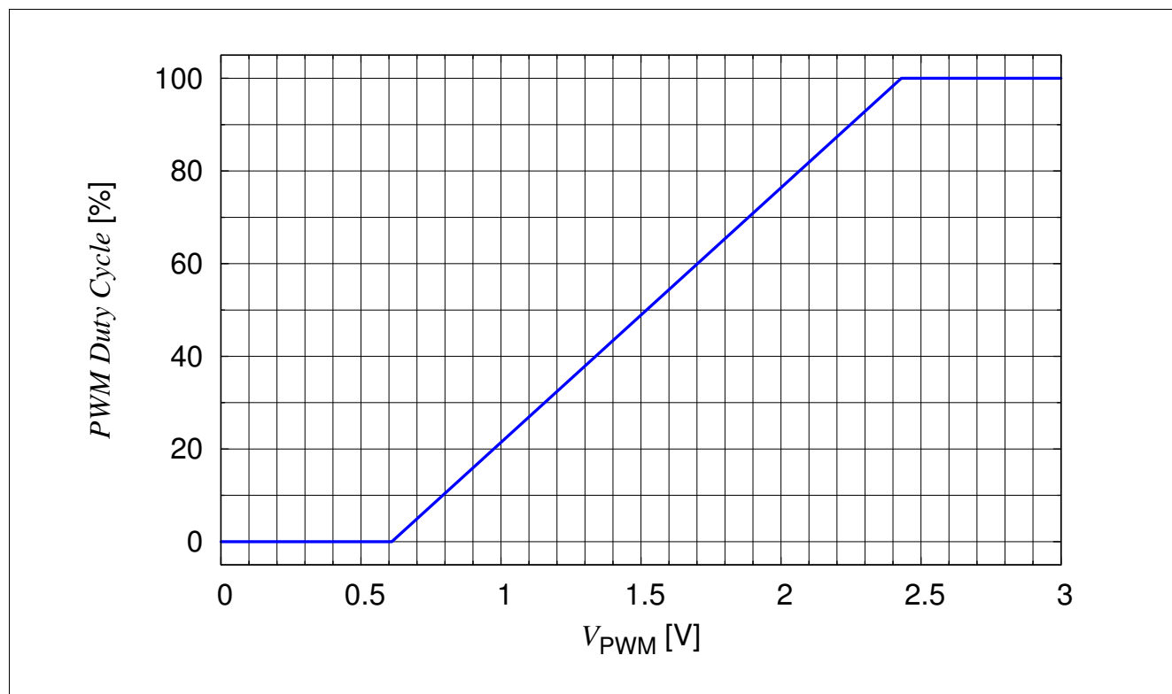
Figure 5 Typical Integrated PWM Duty Cycle vs. PWM Control Voltage
