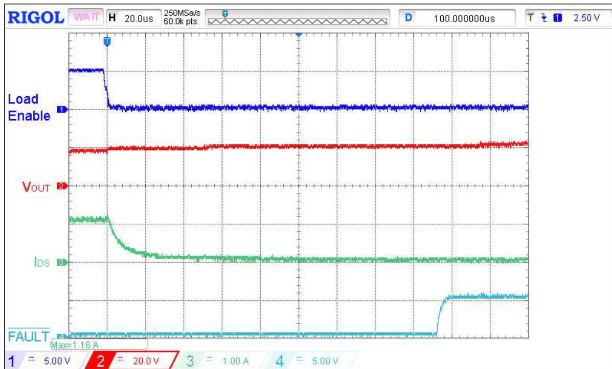
Figure 19. Typical FAULT de-assertion waveform for V_{IN} = 20 V, C_{LOAD} = 10 μF, I_{ACL} = 1 A, R_{SET} = 91 kΩ, switch out 15.6 Ω load
