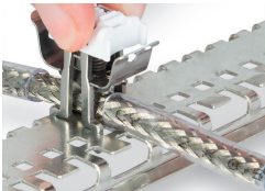
Removing the shield clamping saddle.
