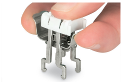
Compress the clamping saddle until fully engaged.
