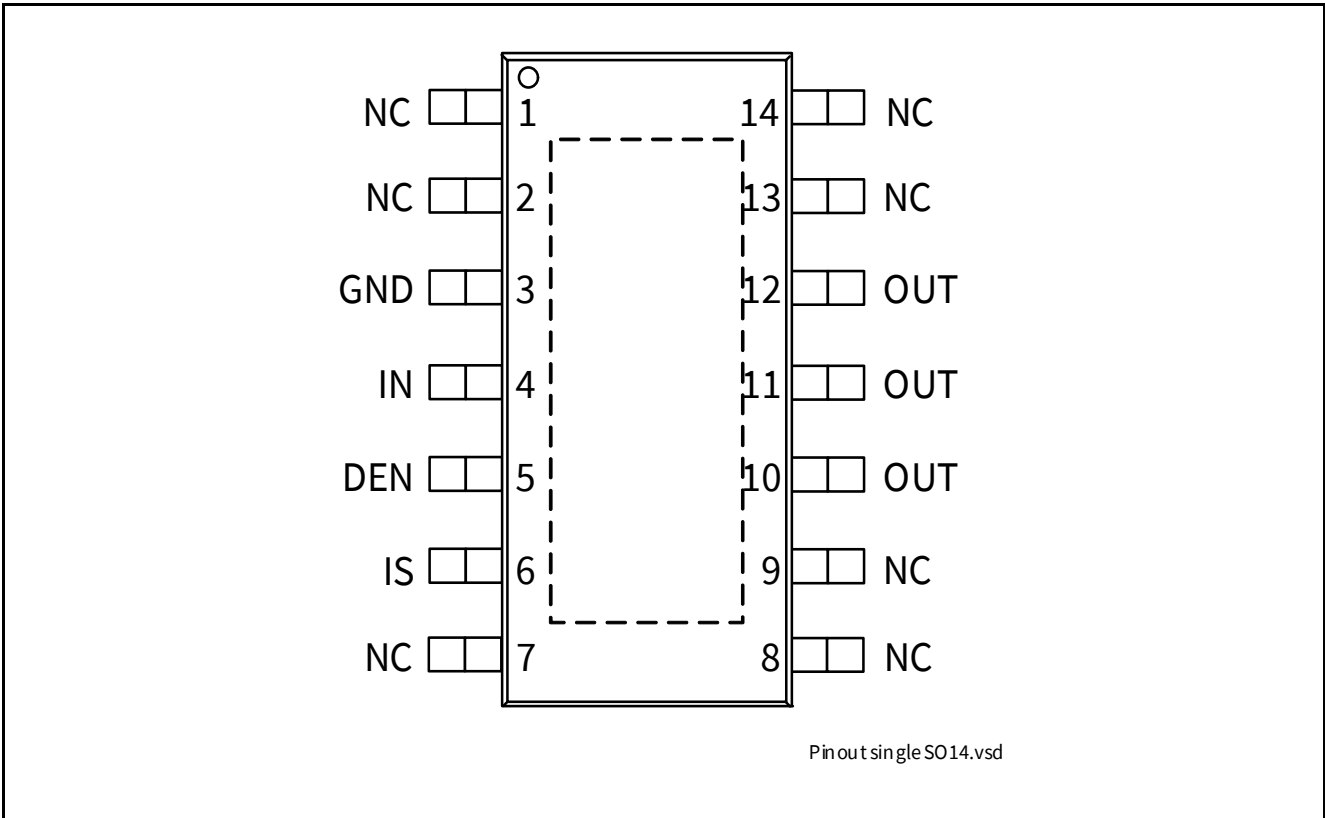
Figure 2 Pin Configuration
