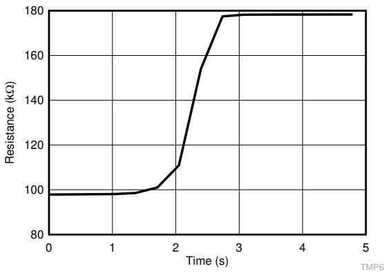
Figure 7-7. Step Response
