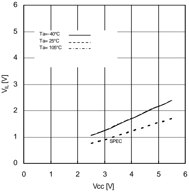
Figure 6. "L" Input Voltage vs Supply Voltage (CSB,SCK,SI,HOLDB,WPB)
