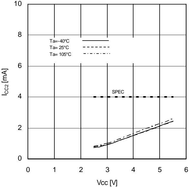
Figure 12 Current consumption at READ operation vs Supply Voltage
