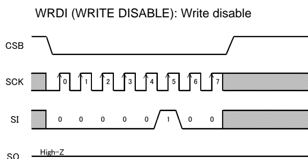
Figure 32. Write disable command
