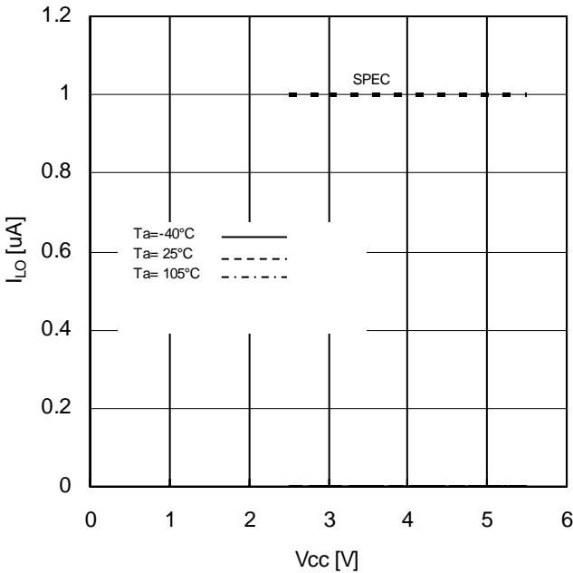
Figure 10. Output Leak Current vs Supply Voltage
