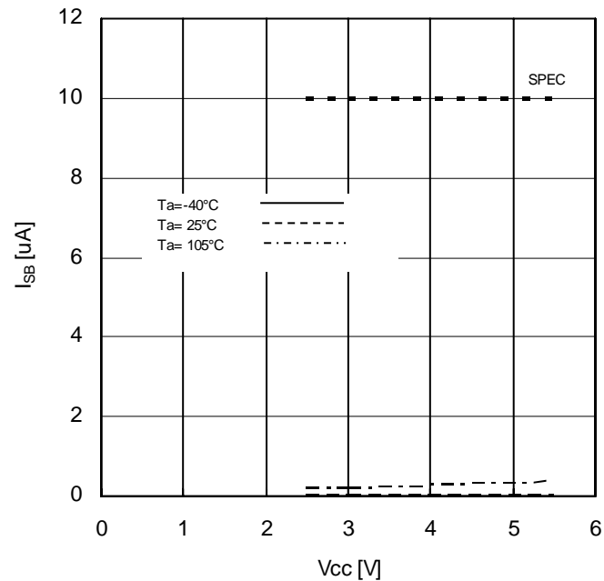
Figure 13. Current consumption at standby operation vs Supply Voltage
