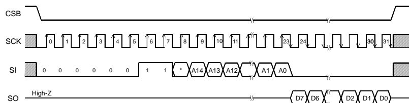
Figure 33. Read command
