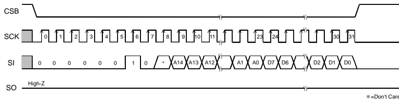
Figure 34. Write command
