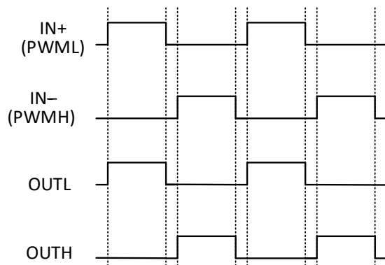
Figure 9: Half-Bridge PWML and PWMH Signals with Dead Time Generated at SOURCE by PWM Controller, AHV85003 and AHV85043 Chipset with Recommended External Transformer
