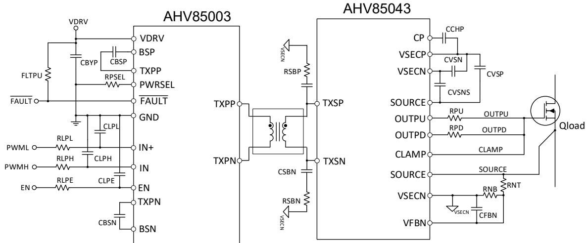
Figure 14: Typical Application Schematic, AHV85003 and AHV85043 Chipset with External Transformer
