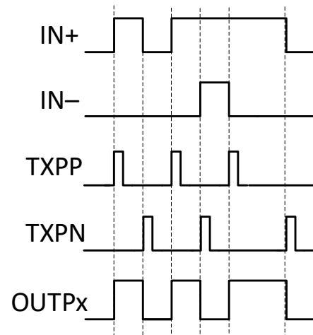
Figure 4: PMW Encoding and Power Transfer
