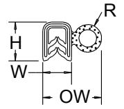
Profile B
