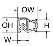
Profile D
