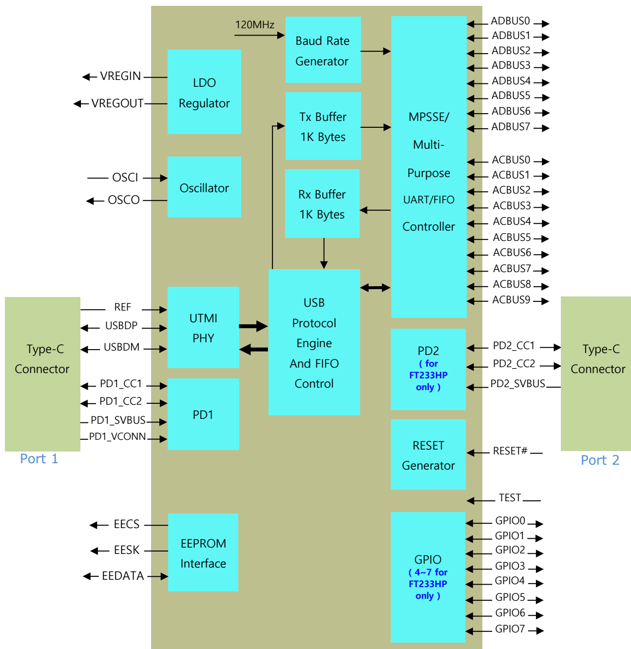
Figure 1 - FT233HP/FT232HP Block Diagram
