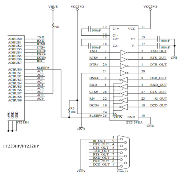
Figure 5 - RS232 Configuration
