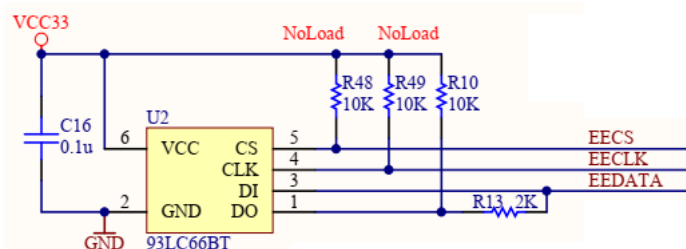
Figure 37 - EEPROM Interface
